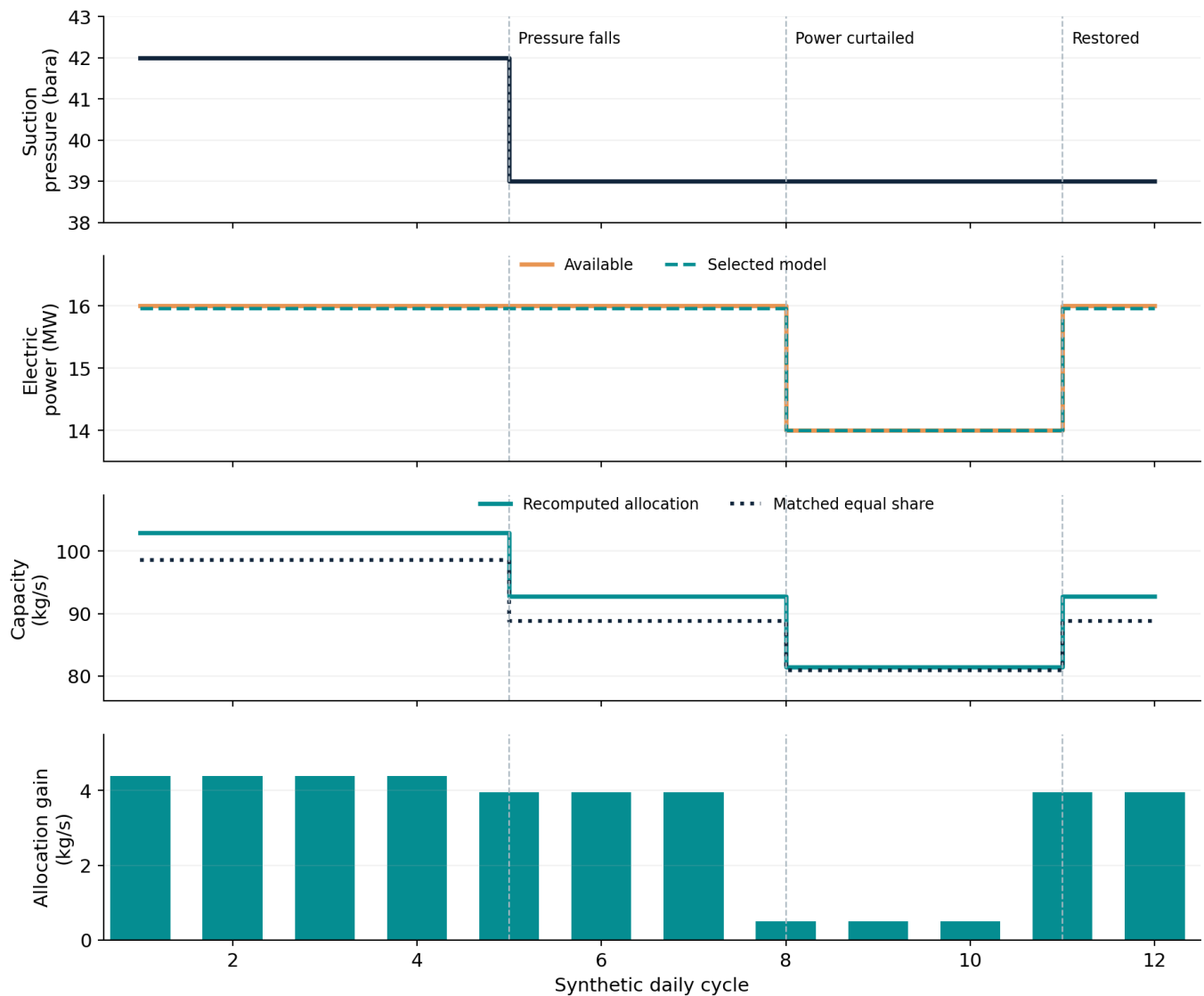
Figure 18. Executed synthetic live replay. Pressure and power allocation are inputs; electrical demand and throughput are recomputed with NeqSim. The lower panel reports allocation gain against a reference at matching conditions. Event lines identify prescribed input changes, not measured alarm lead times.
