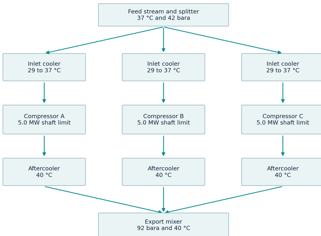
Figure 16. The exact equipment connectivity built by the accompanying script: one feed and splitter, three cooler-compressor-aftercooler branches, and an export mixer. Pipe and cooler pressure losses are neglected in this screening model.
