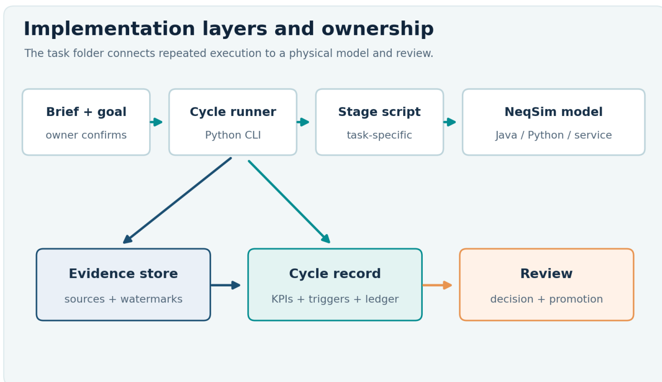
Figure 4. The runner controls time and records; the model computes; the agent handles exceptions; the reviewer controls acceptance.
